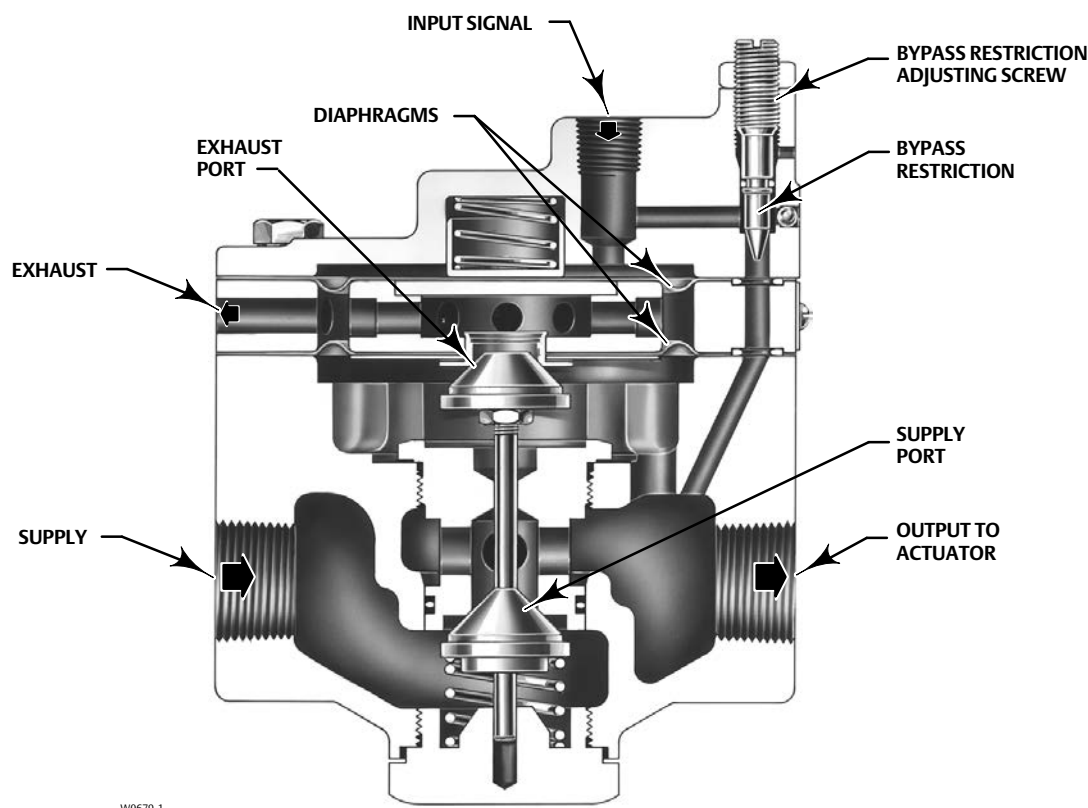
Figure 1. Sectional View of Volume Booster
