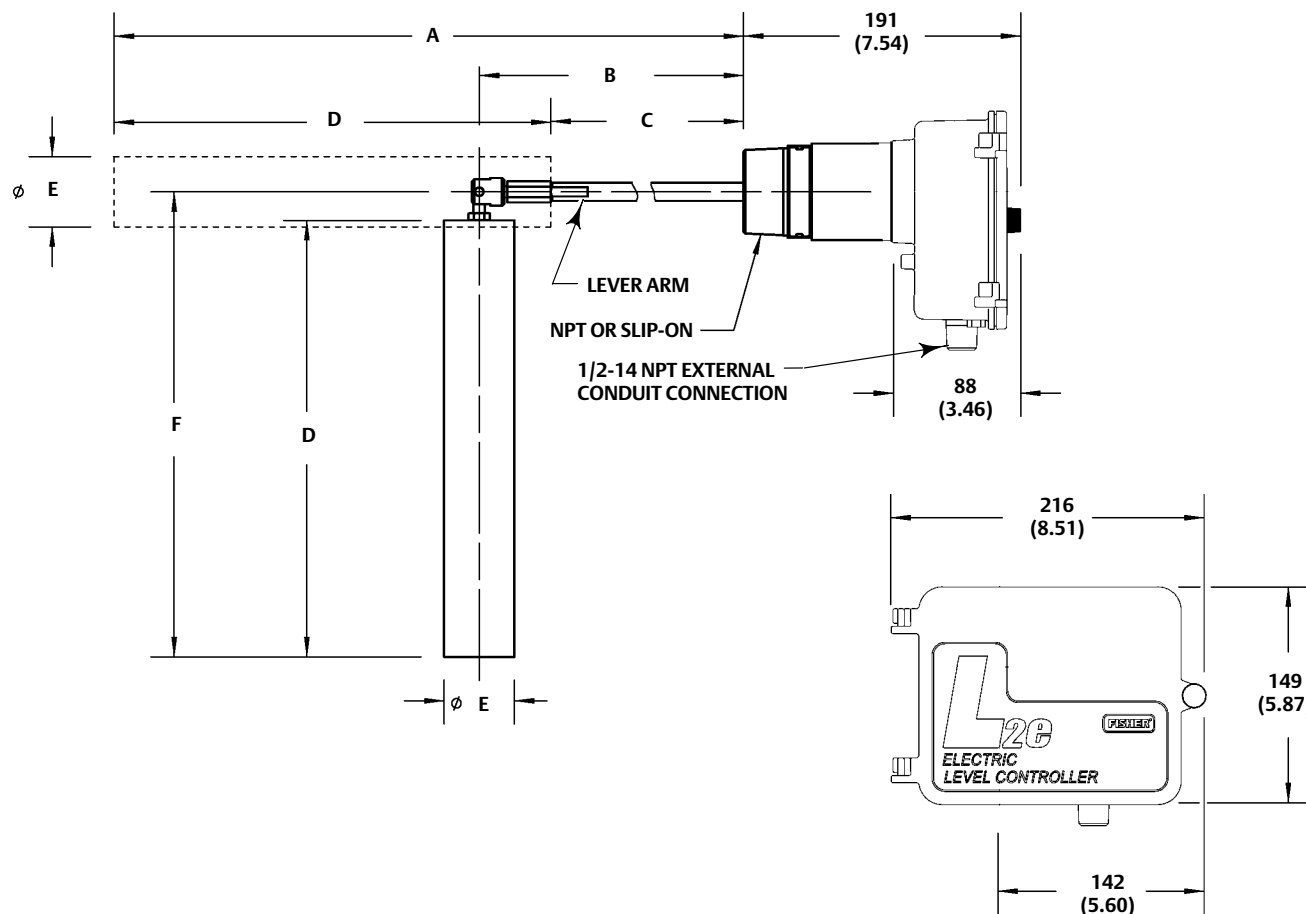
Figure 2. Dimensions
